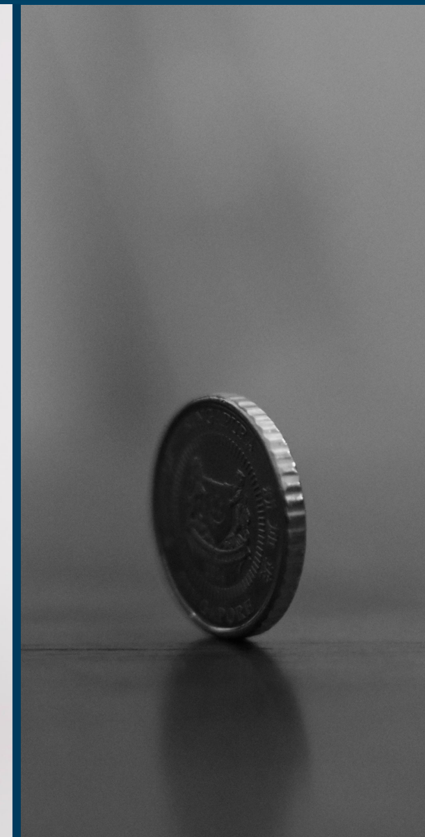
4. Statistical Prediction
