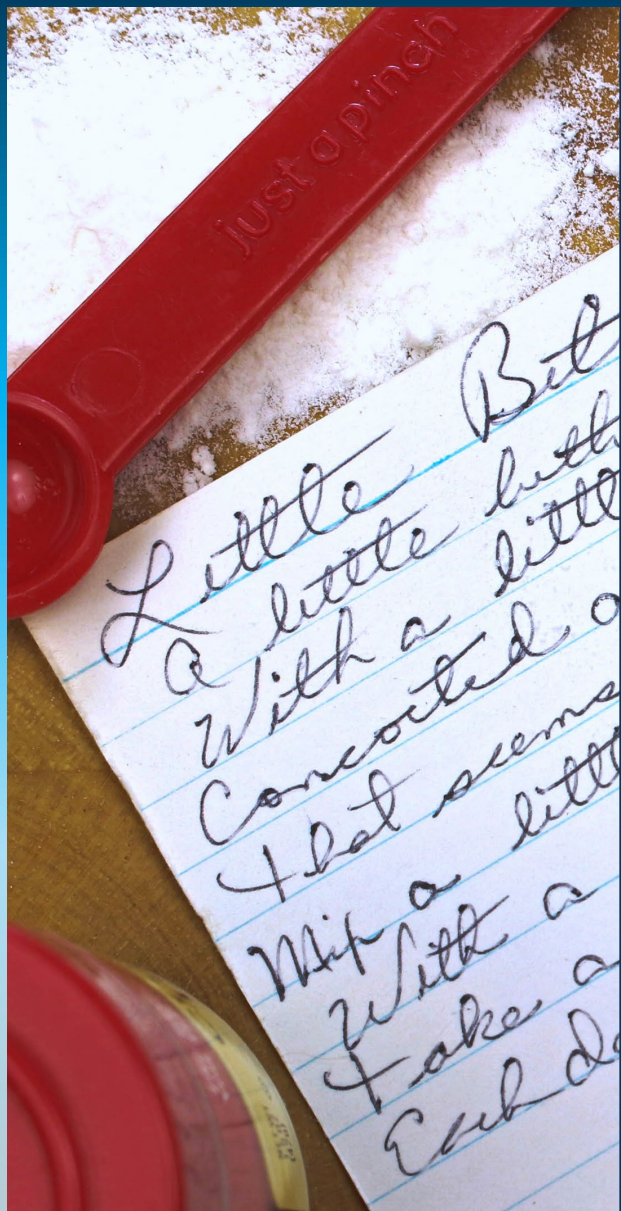
1. Sequential
